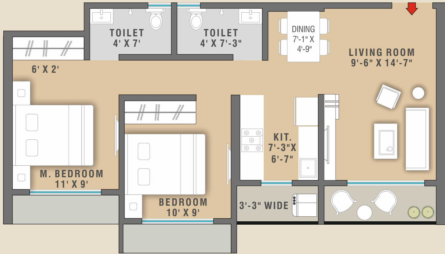
Unit Plan
